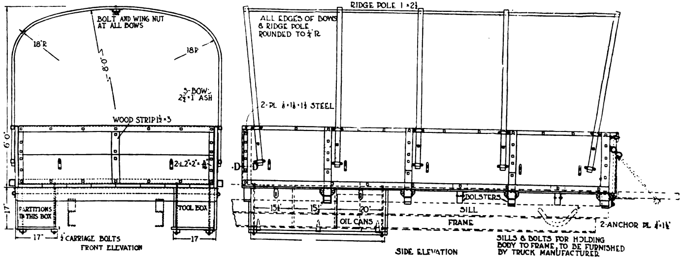
CLASS B MILITARY TRUCK
